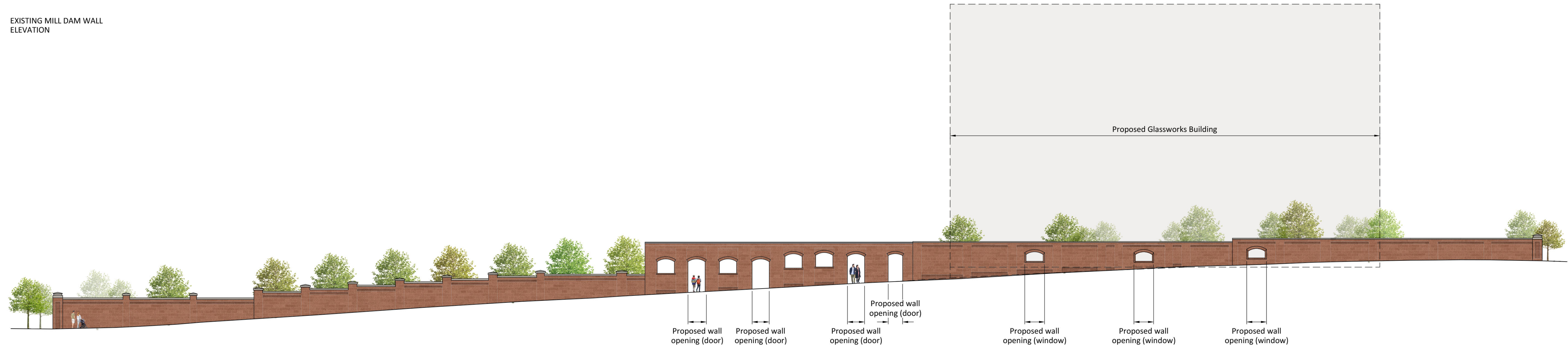
PROPOSED MILL DAM WALL ELEVATION
